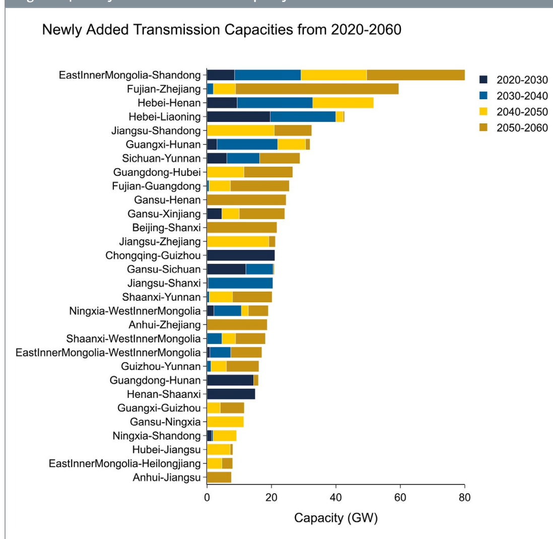
Figure 7 | Newly Added Transmission Capacity from 2020 to 2060
