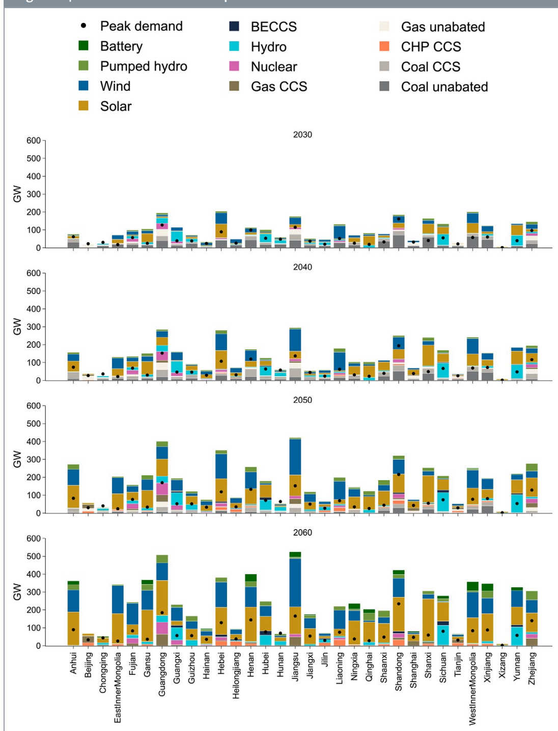
Figure 6 | Provincial Generation Capacities from 2030 to 2060
